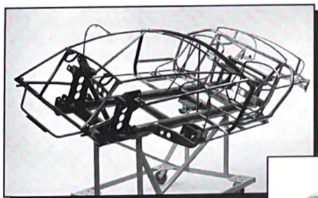
HI-TECH 427SC ROADSTER CHASSIS
